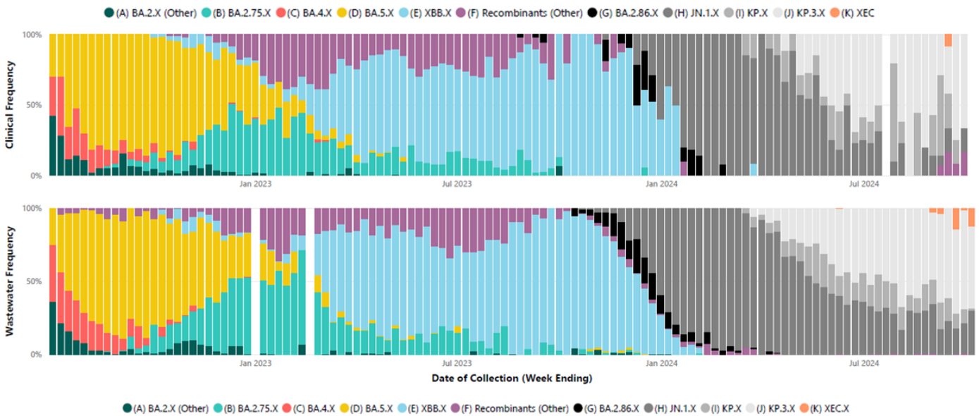
Figure 12. Distribution of SARS-CoV-2 variants in clinical samples (top) and metropolitan wastewater catchments (bottom), 03 July 2022 to 6 October 2024.
