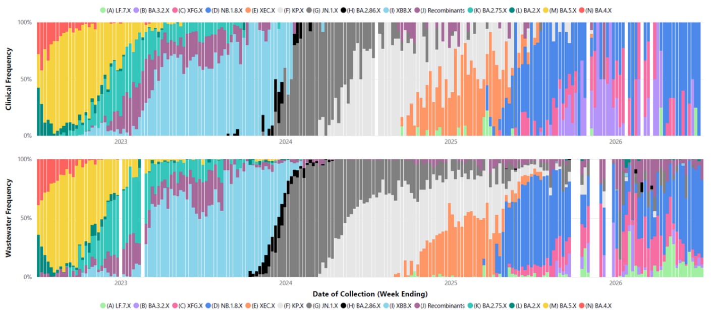
Figure 18. Distribution of SARS-CoV-2 variants in clinical samples (top) and metropolitan wastewater catchments (bottom), 3 July 2022 to 12 July 2026
