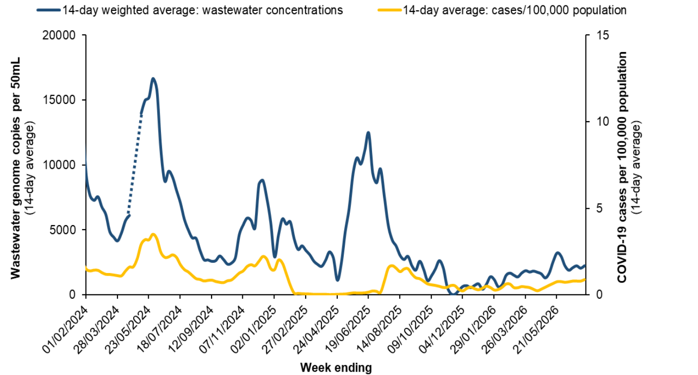
Figure 17. SARS-CoV-2 concentration in wastewater and COVID-19 notification rate, Perth metropolitan area, WA, 2024 to 10 July 2026.
